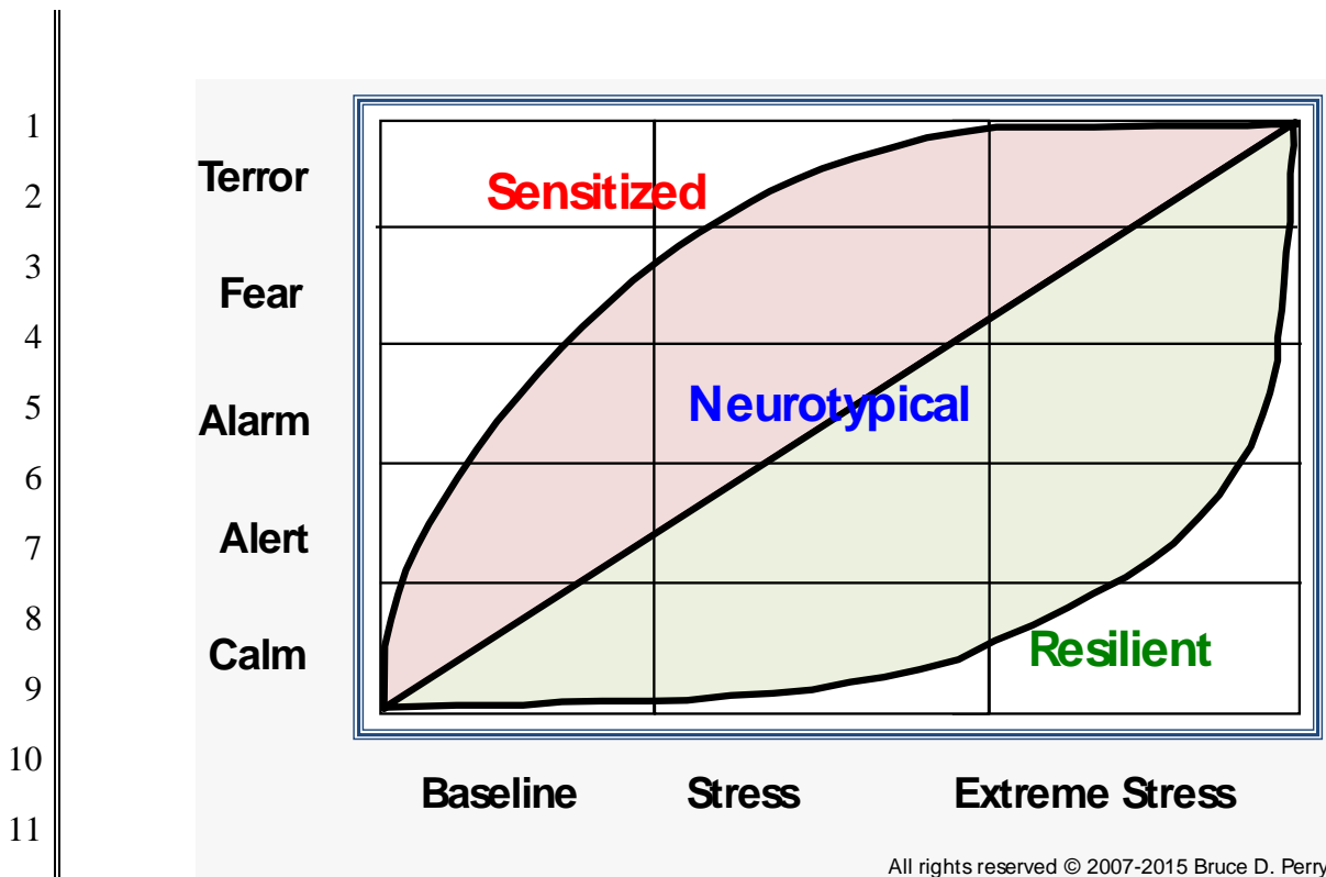
Figure 6. Differential Stress-Reactivity
